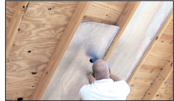
Gorell R-Comfort Rafter Wrap installs easily and quickly. For R-Comfort Rafter Wrap T applications, simply staple the insulation tab to the inside of the rafters.
